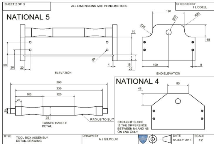
Orthographic Drawing
